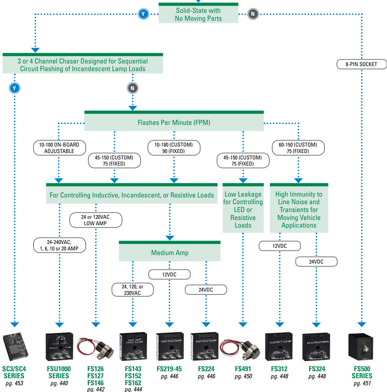
Flashers
