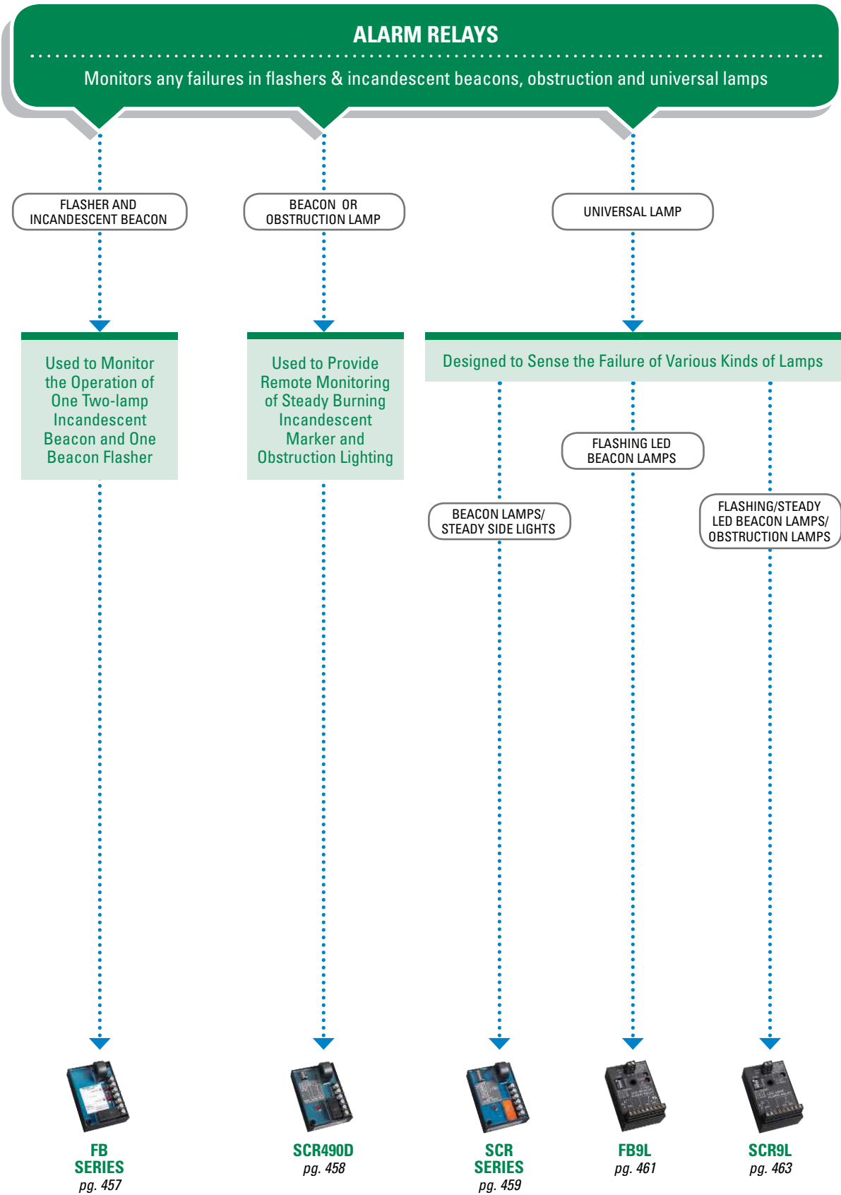
Alarm Relays
